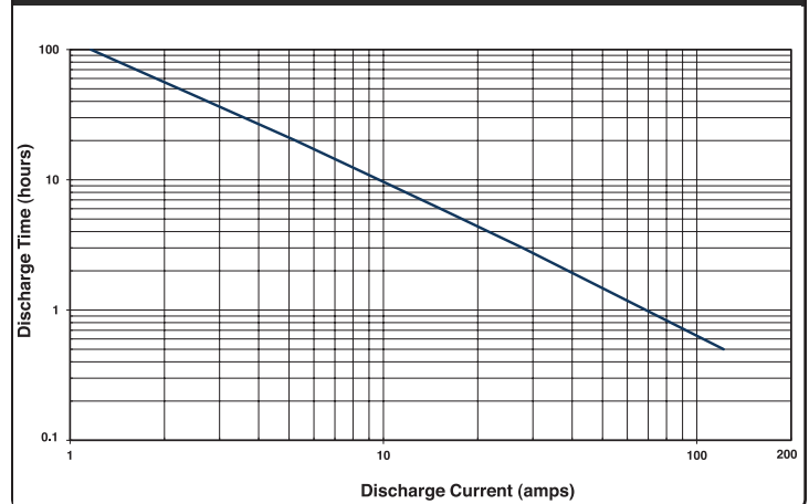
US 27DC XC2 DISCHARGE TIME VS CURRENT @80° F
